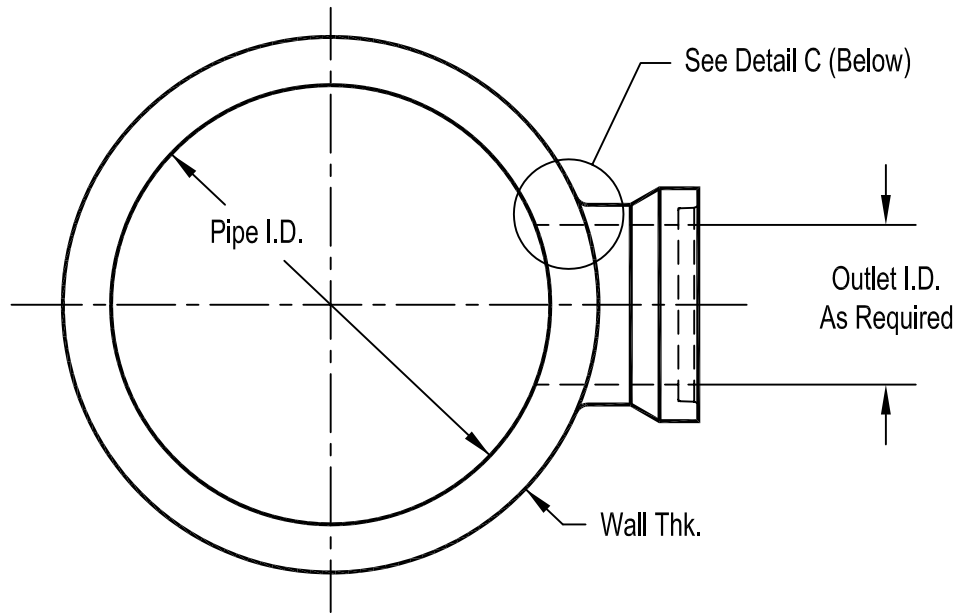
View Looking From Spigot To Bell
