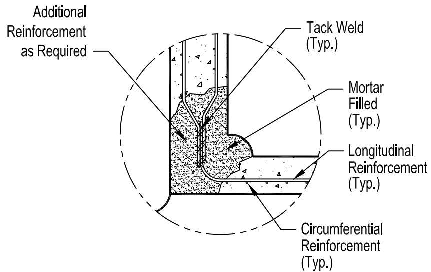
Detail C
