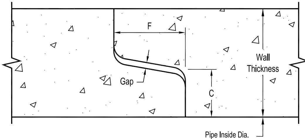
Section Thru Joint
